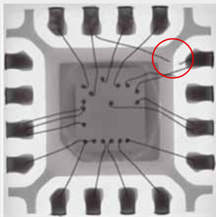
Broken bond wire
