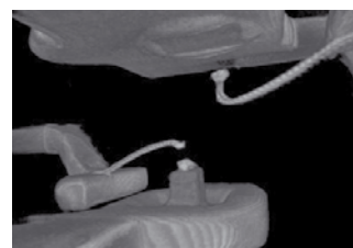
CT provides a 3D image of a broken bond wire
